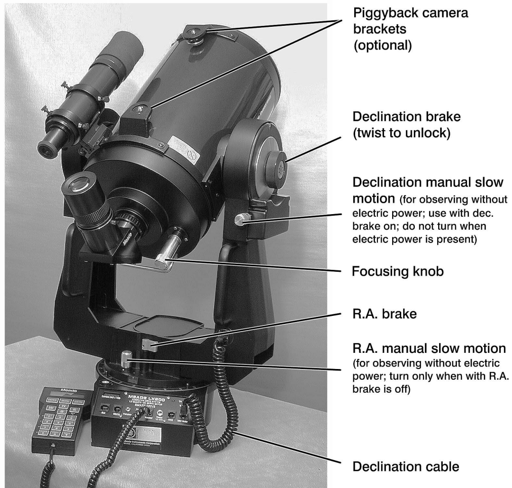
Figure 10.1: Important parts of an LX200 telescope.
